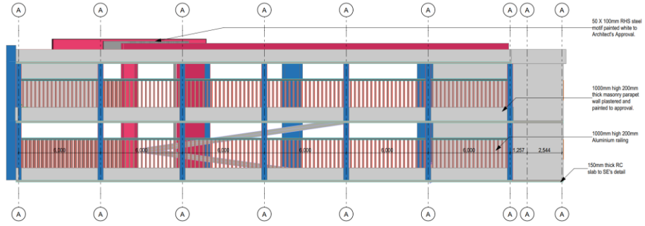
ELEVATION 03 SCALE 1:100
