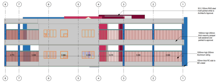
ELEVATION 02 SCALE 1:100
